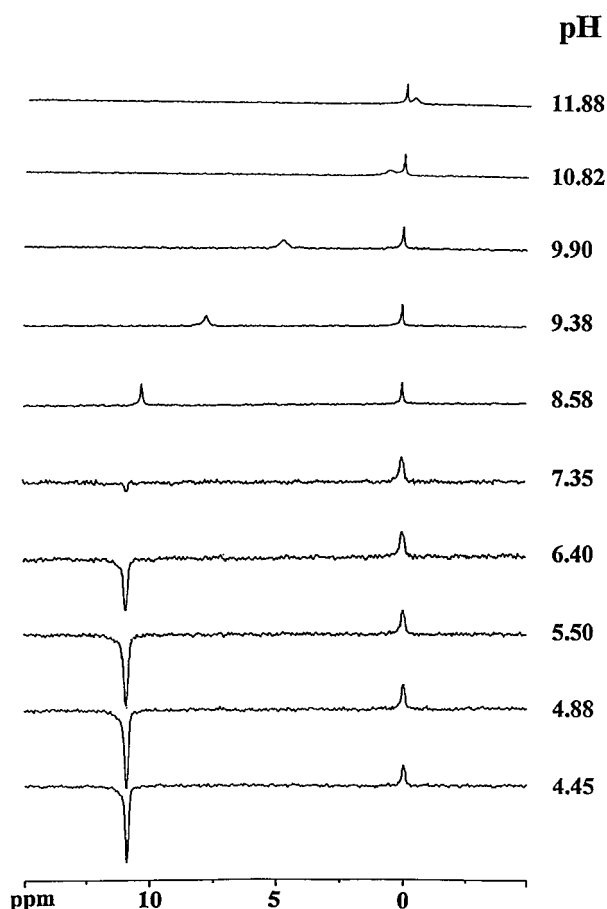
FIGURE 1 ^{15}N NMR spectra of 48 mM [^{15}N] Gly in 50 mM sodium phosphate and 100 mM NaCl as a function of pH. ^{15}NH_4NO_3 in D_2O in the inner NMR tube of coaxial NMR tubes was used as a reference.
